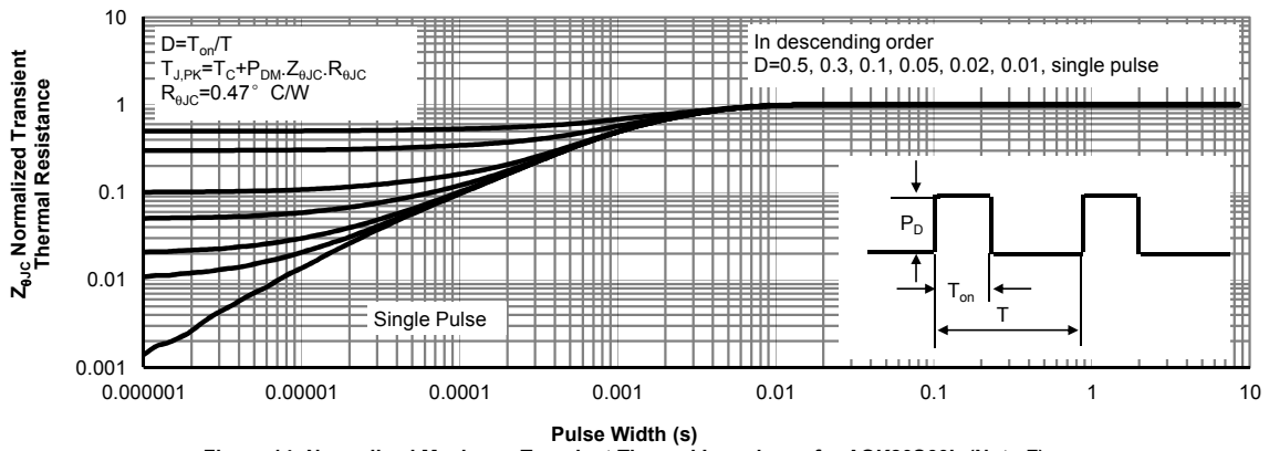
Figure 14: Normalized Maximum Transient Thermal Impedance for AOK20S60L (Note F)
