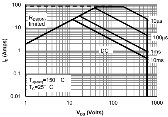
Figure 11: Maximum Forward Biased Safe Operating Area for AOK20S60L (Note F)
